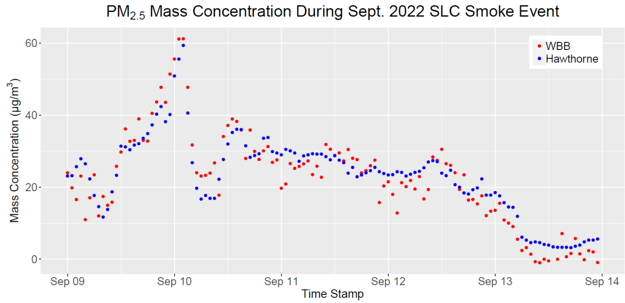
Figure 1. Graph of PM 2.5 mass concentration data from both WBB and Hawthorne Elementary TEOM instruments during 5-day September 2022 smoke event in Salt Lake City area.
