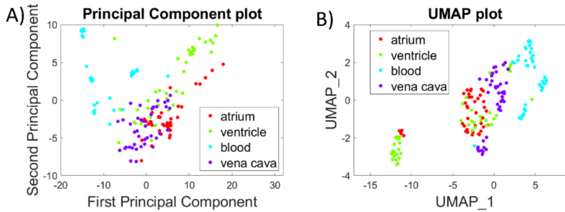
Figure 1: Dimensionality reduction approaches used on the spectral data. The colors correspond to the tissue type. A) Plot of the principal components yielded a separation of blood from tissue as well as separation of certain tissue regions. B) UMAP plot revealing distinctions between blood and tissue, but also differences in some of the ventricle regions vs. other sites
