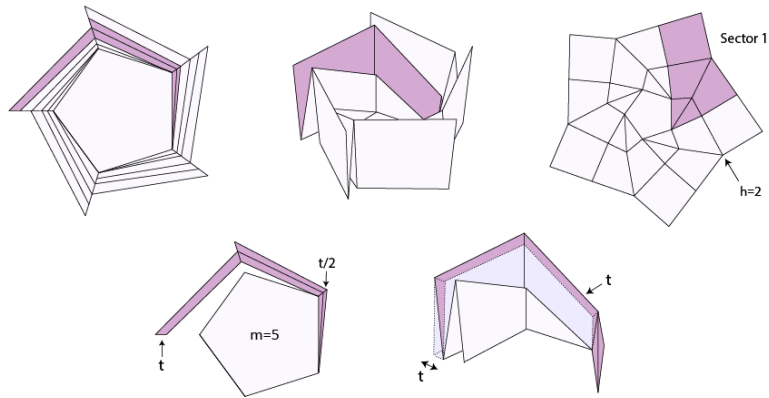
Figure 1: The m5-h2-r1 flasher pattern is illustrated with one repeating sector highlighted.
