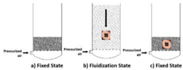
Figure 1. Fluidized Bed in fixed state and fluidized state.
